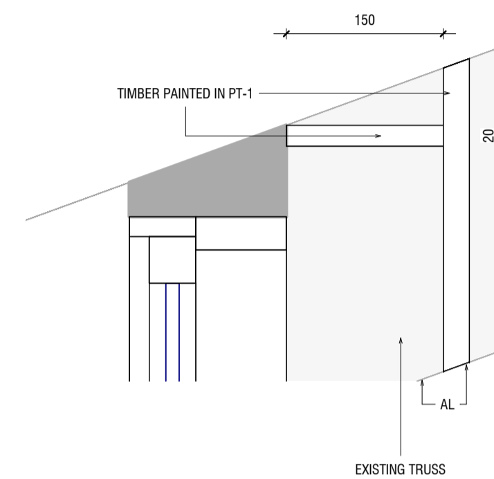
2 TYPICAL TIMBER PELMET - SECTION 1:5
