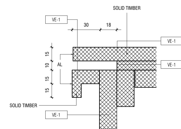
6 TV ROOM DRAWER HANDLE - SECTION 1:2
