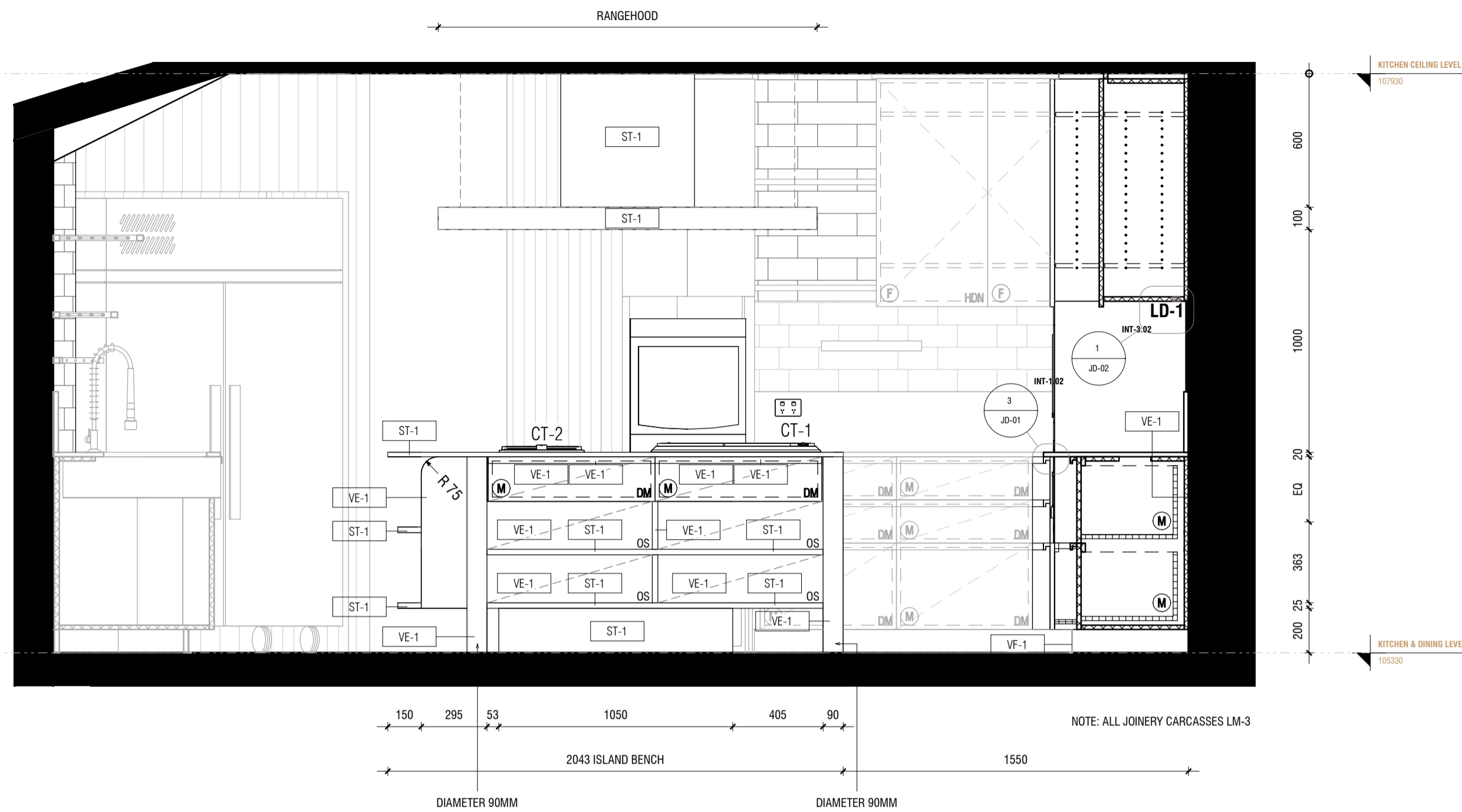
1 INT-3.03 KITCHEN ELEVATION 1 1:20
