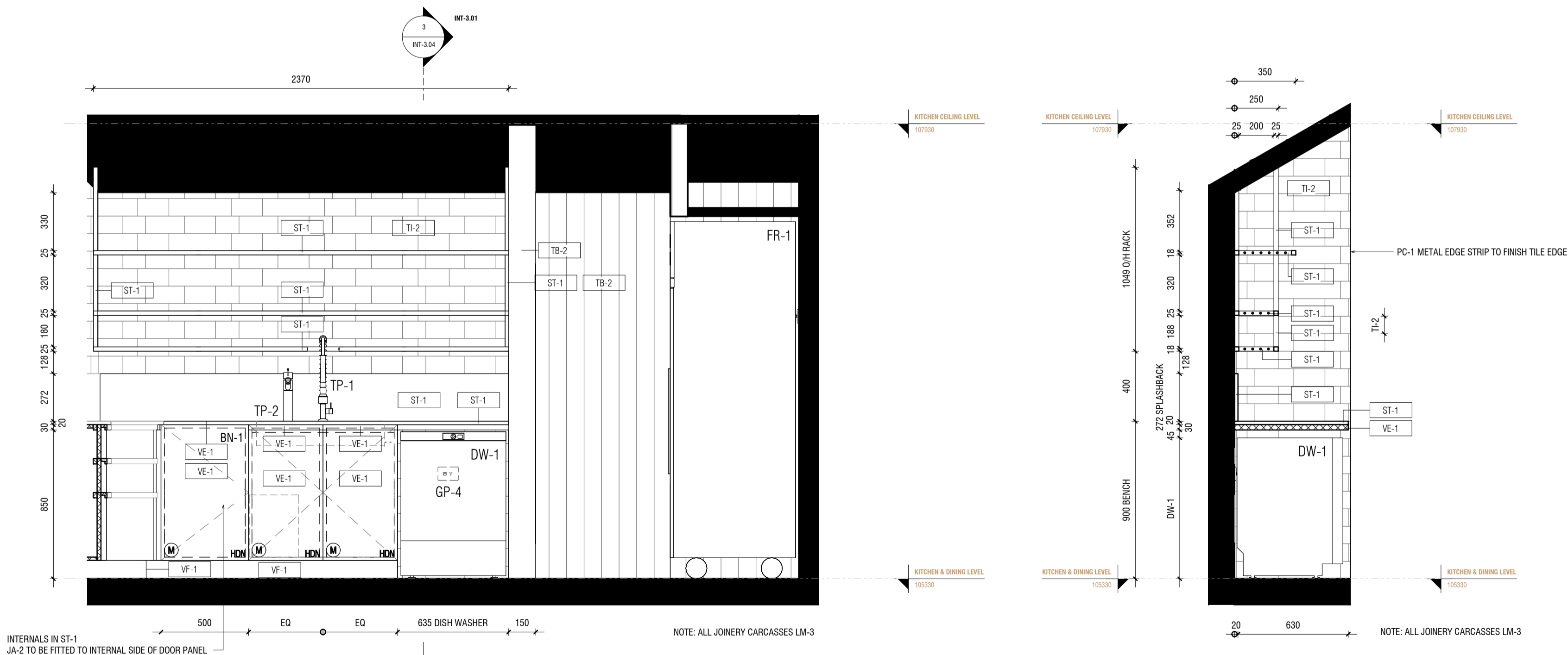
2 INT-3.04 KITCHEN ELEVATION 2 1:20
