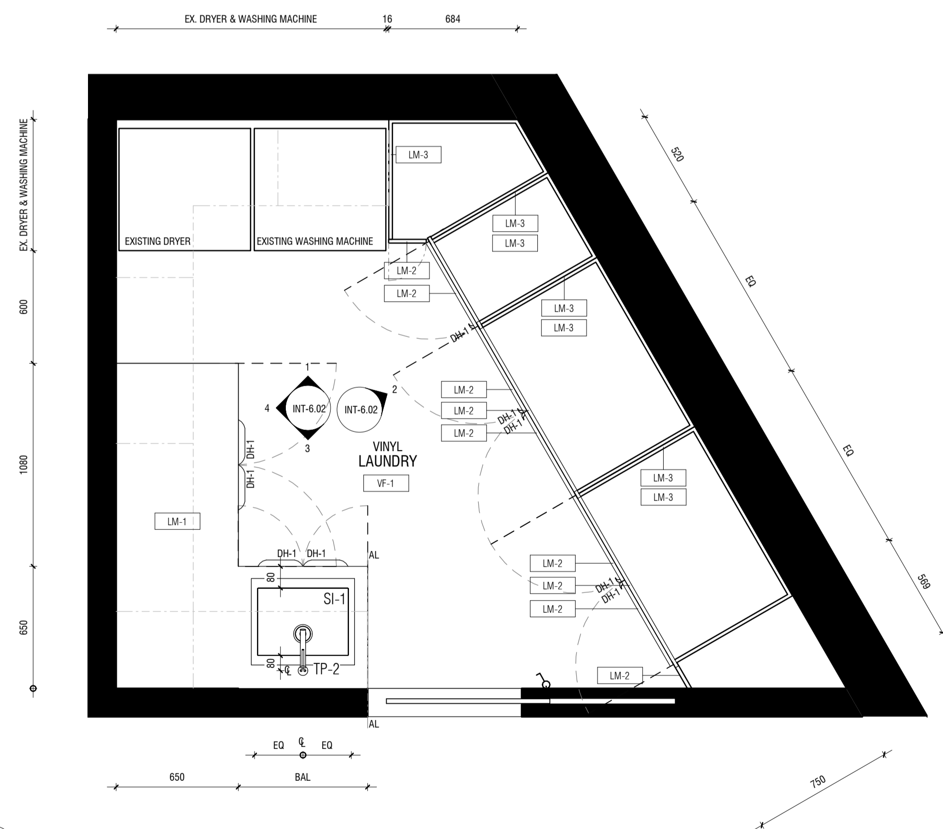
1 LAUNDRY FLOOR PLAN 1 : 20
