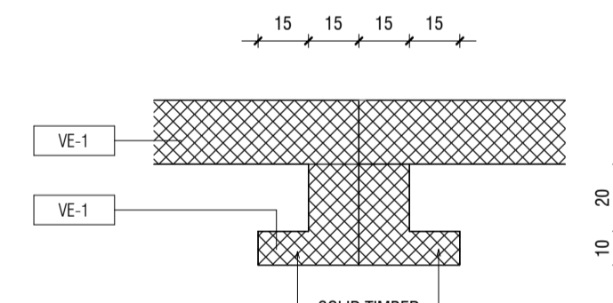
7 TV ROOM TALL UNIT HANDLE - PLAN 1:2
