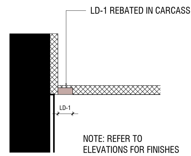
1 TYPICAL LED STRIP LIGHTING - SECTION 1:5
