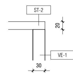
6 BEDROOM DRAWER - ELEVATION 1:5
