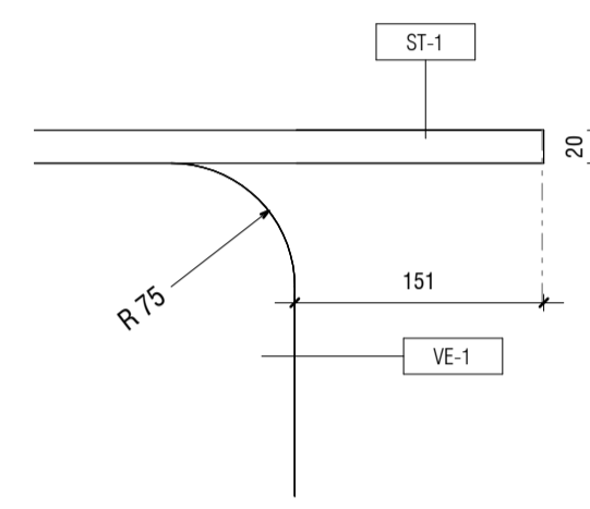
2 KITCHEN ISLAND BENCH - ELEVATION 1:5
