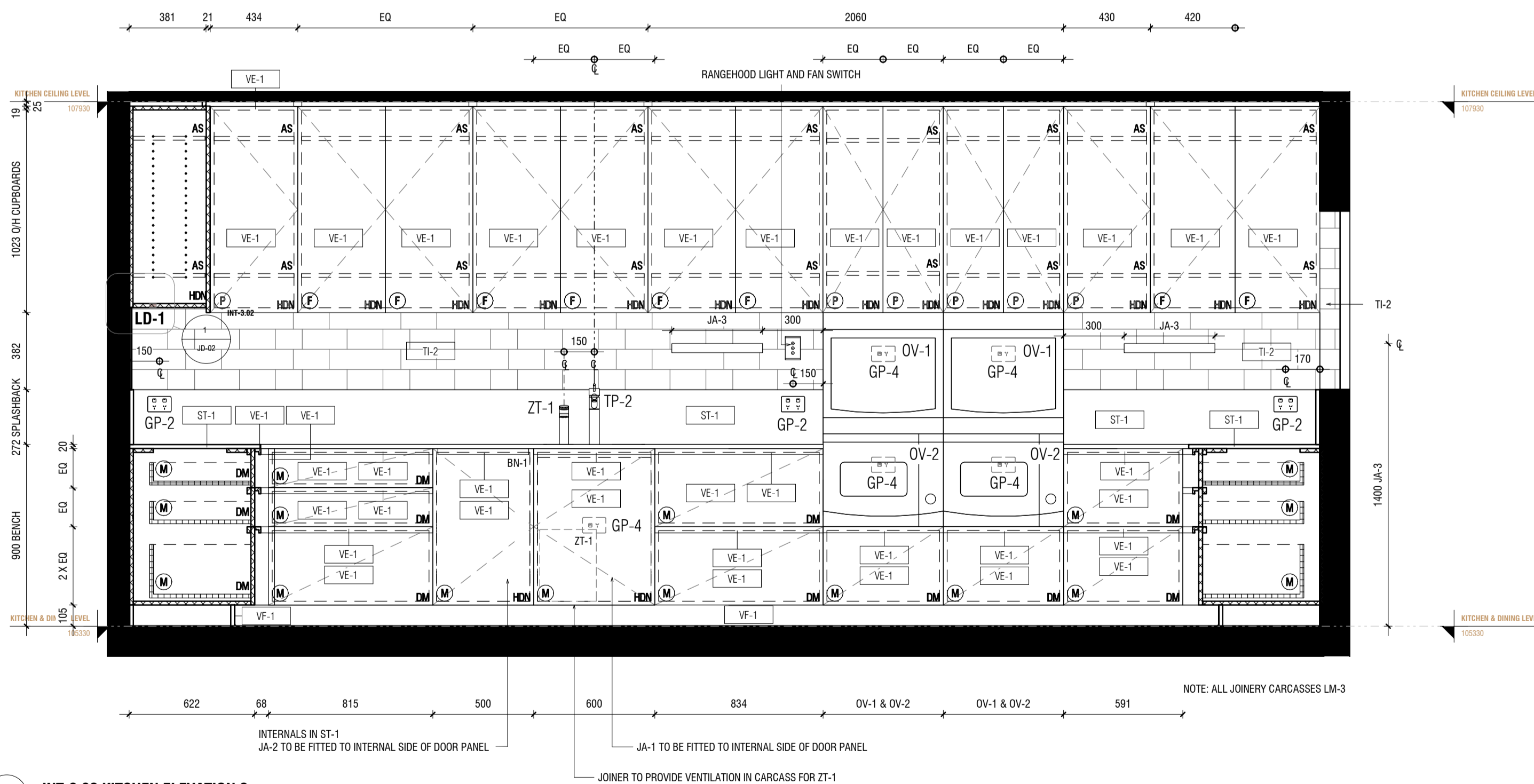
2 INT-3.02 KITCHEN ELEVATION 2 1 : 20
