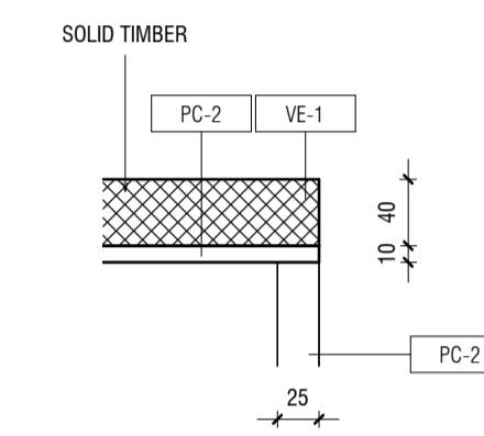
4 WOOD STORAGE - SECTION 1:5
