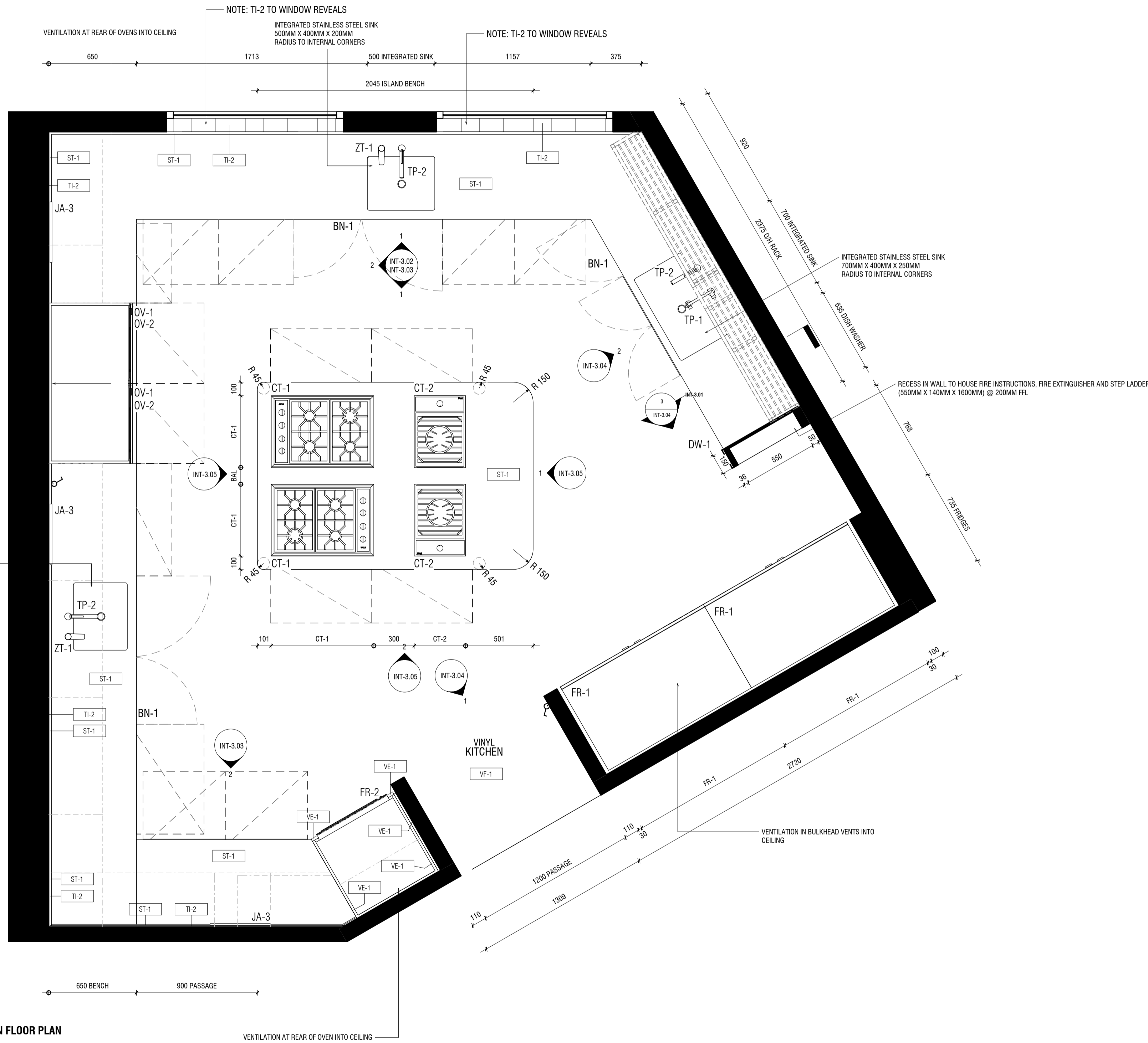
1 KITCHEN FLOOR PLAN 1 : 20
