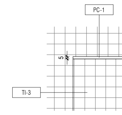
4 TYPICAL ENSUITE SHOWER SHELF - ELEVATION 1:5
