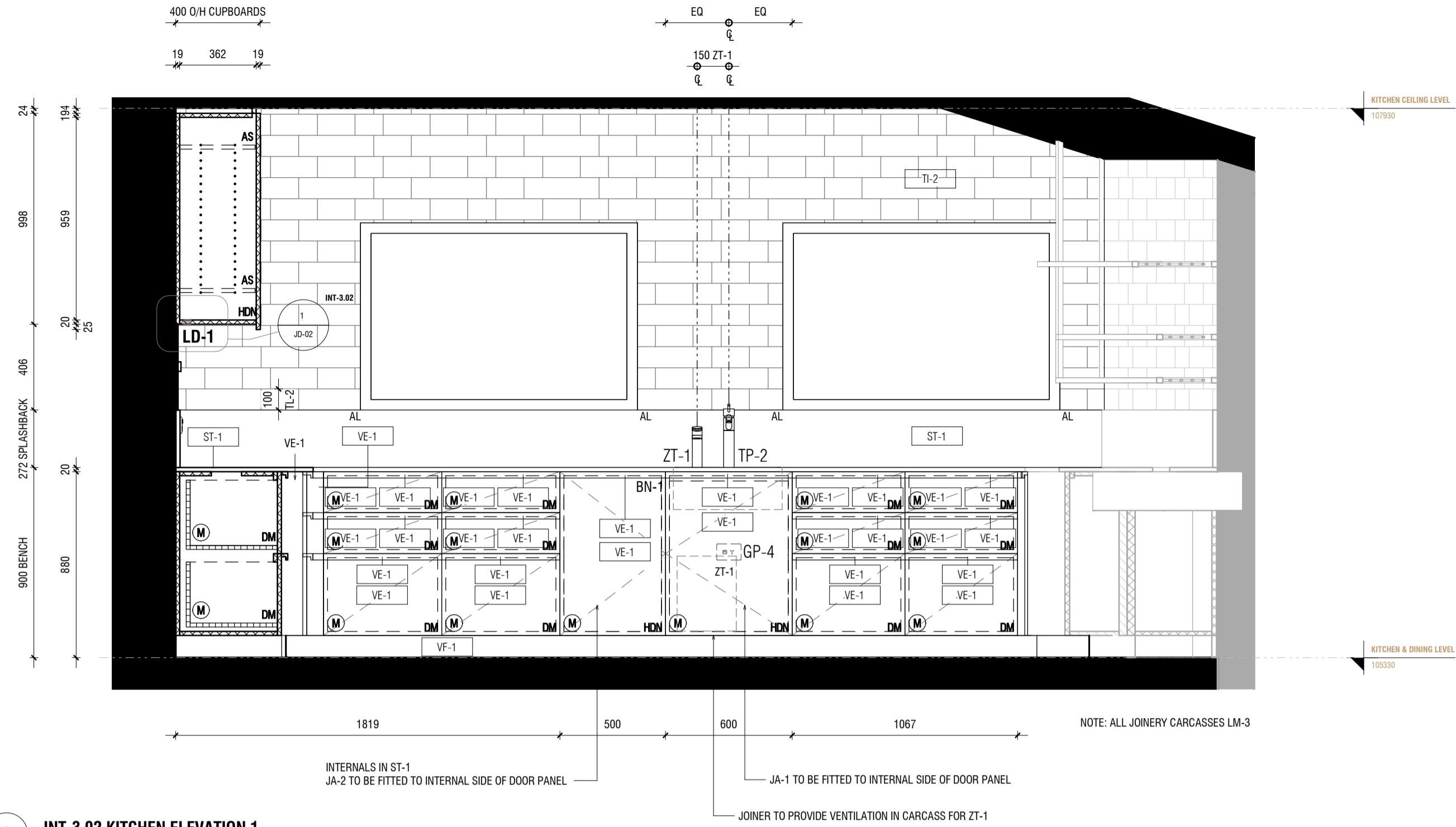
1 INT-3.02 KITCHEN ELEVATION 1 1 : 20
