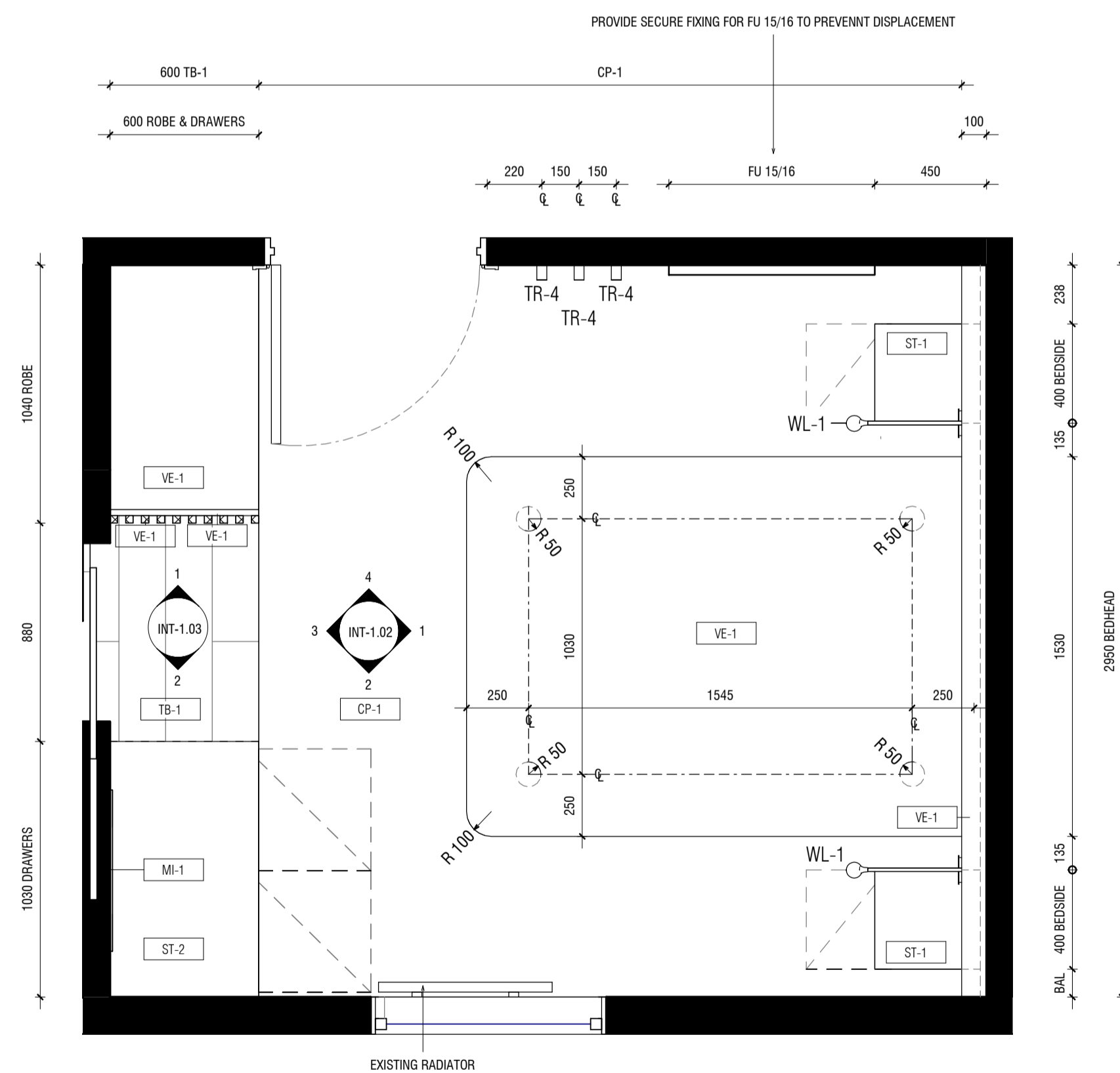
1 TYPICAL BEDROOM FLOOR PLAN 1:20
