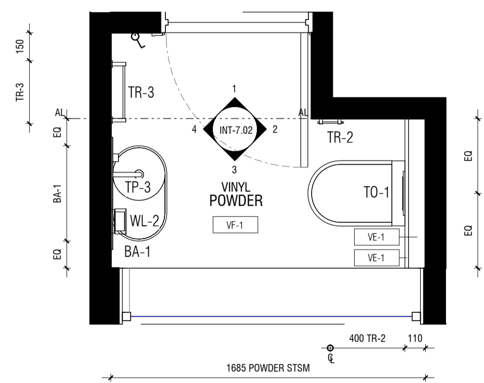
1 POWDER FLOOR PLAN 1 : 20
