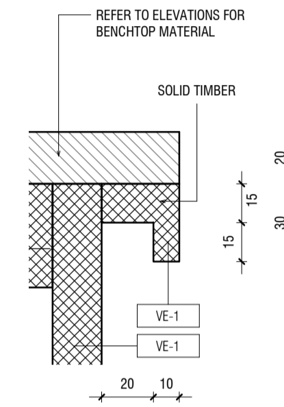
3 TYPICAL DRAWER HANDLE - SECTION 1:2
