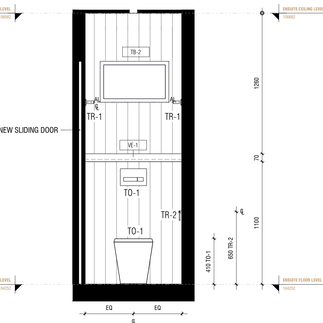
2 INT-2.01 TYPICAL ENSUITE ELEVATION 2 1 : 20
