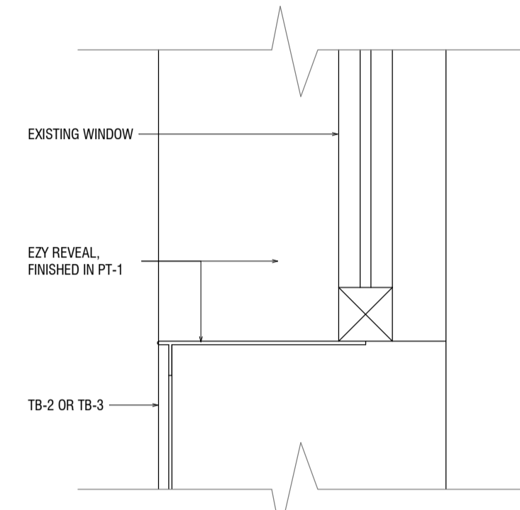
3 TYPICAL WINDOW REVEAL - SECTION 1:5
