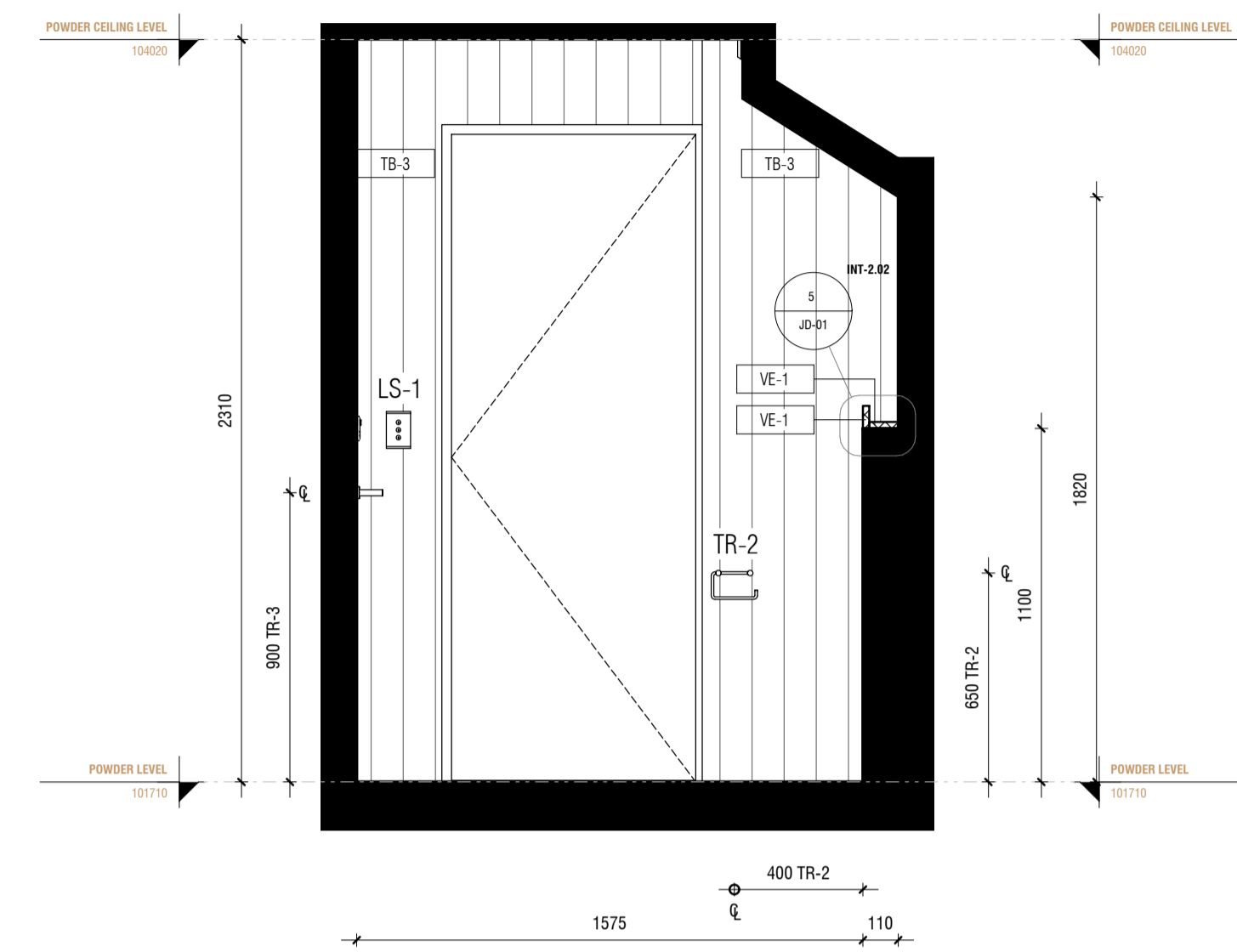
1 INT-7.02 ELEVATION 1 1:20
