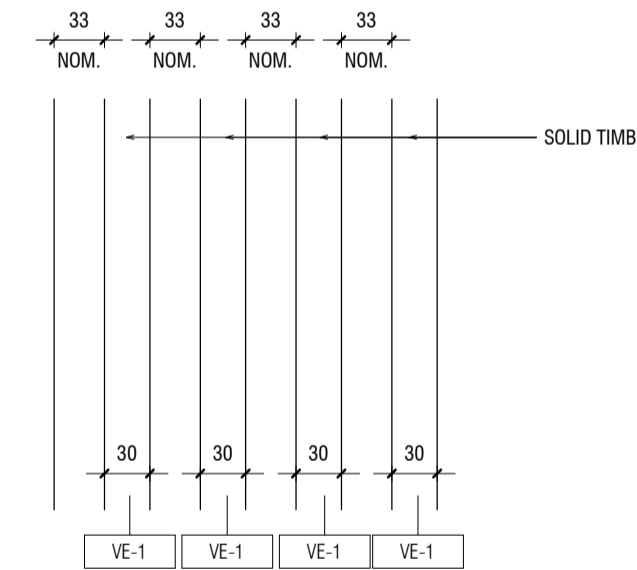
7 TYPICAL ROBE/DRAWERS - ELEVATION 1:5
