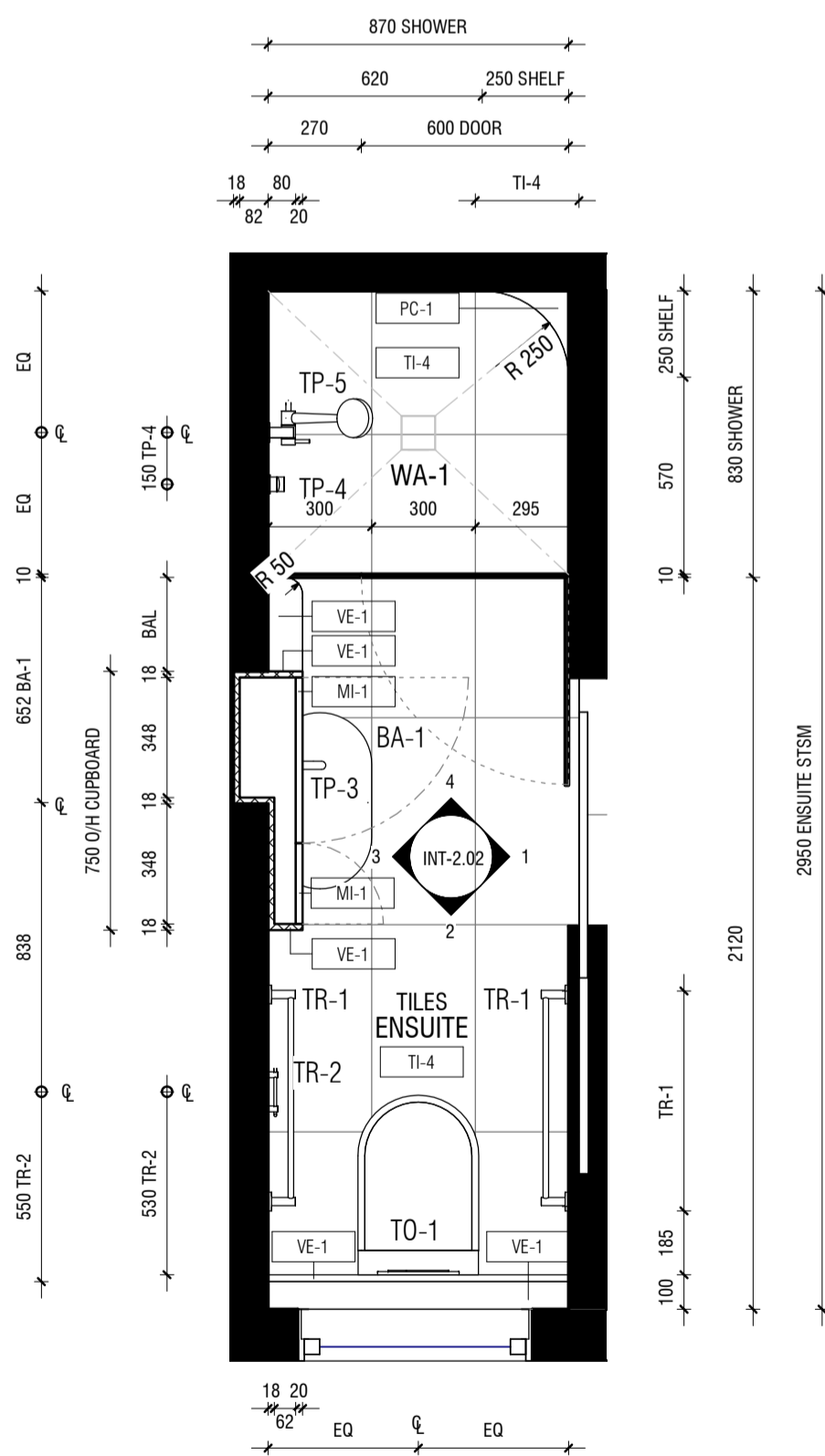
1 TYPICAL ENSUITE FLOOR PLAN 1 : 20
