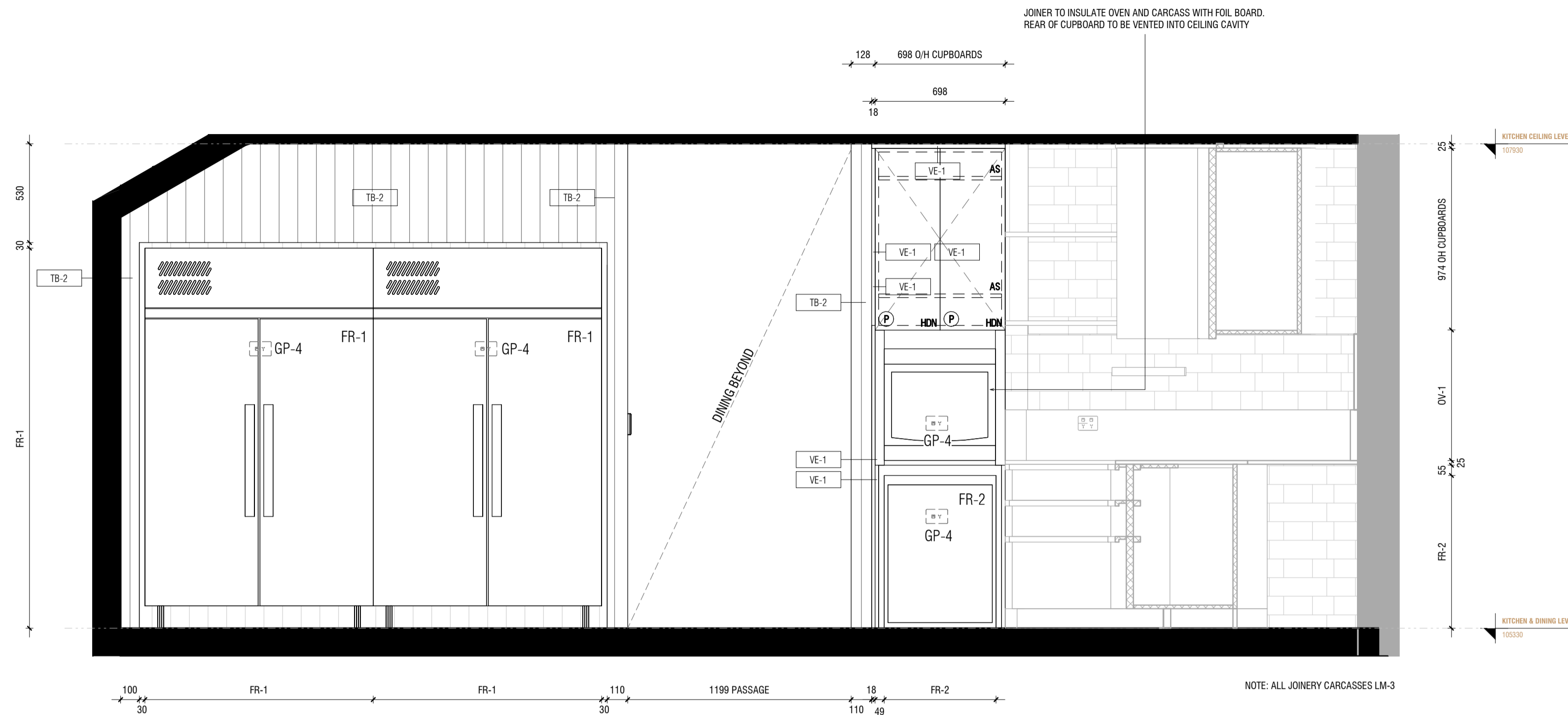
1 INT-3.04 KITCHEN ELEVATION 1 1:20
