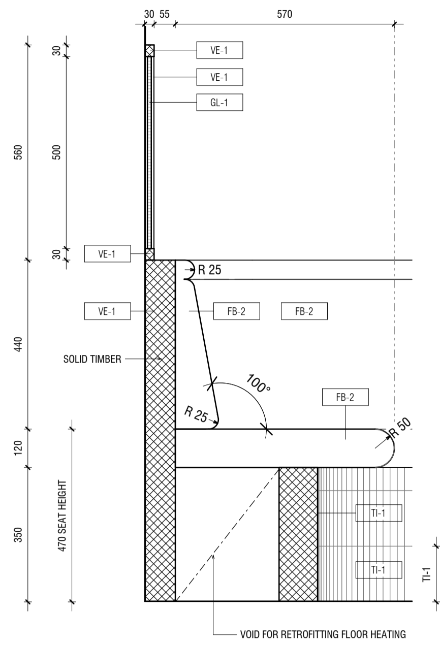
1 BANQUETTE SEAT - SECTION 1:10
