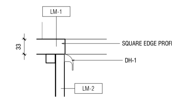
8 LAUNDRY BENCHTOP PROFILE - SECTION 1:5
