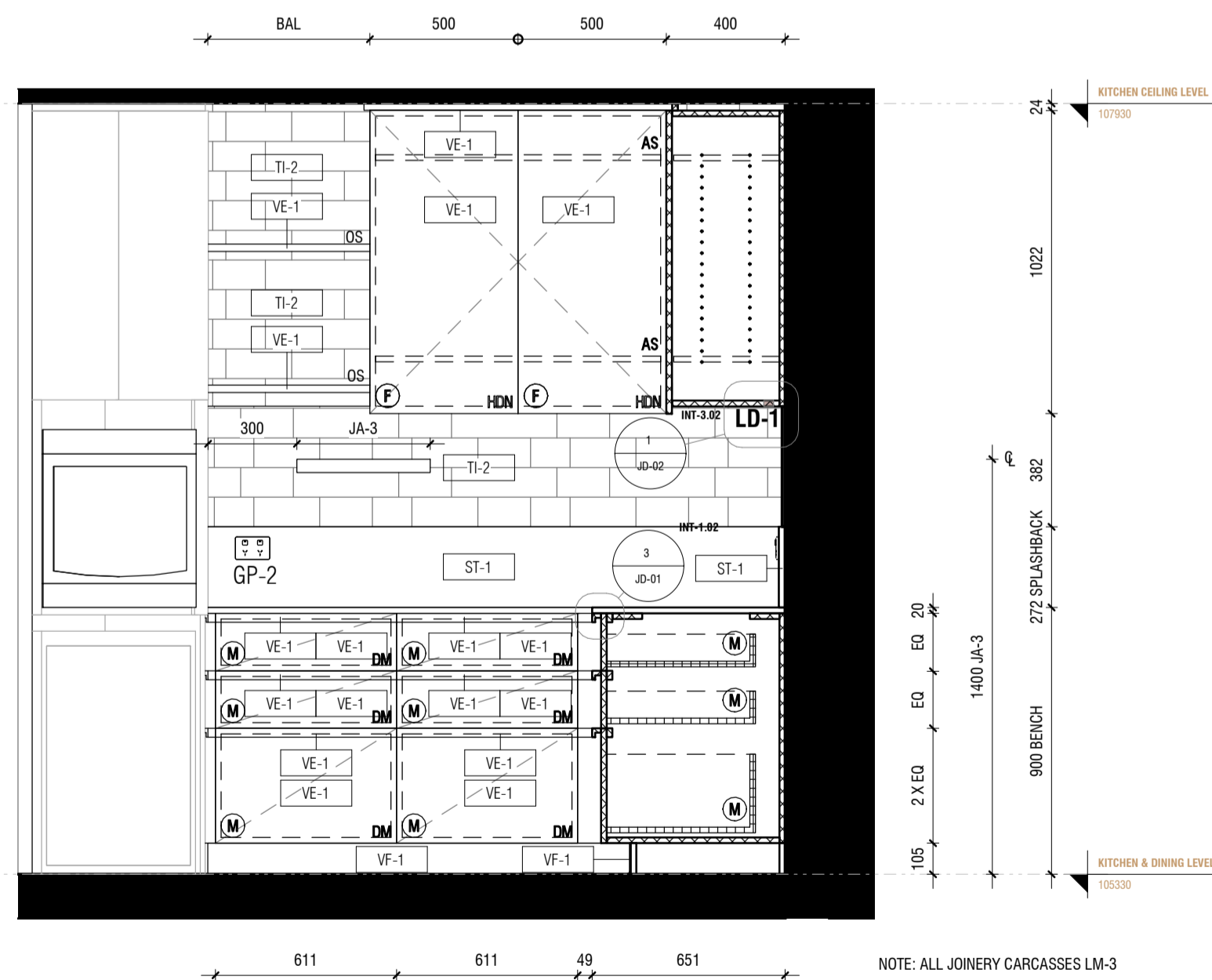
2 INT-3.03 KITCHEN ELEVATION 2 1:20
