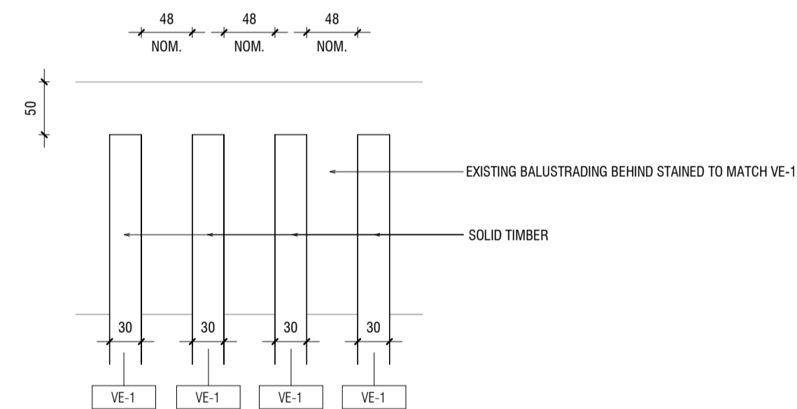
5 TYPICAL BALUSTRADE - ELEVATION 1:5
