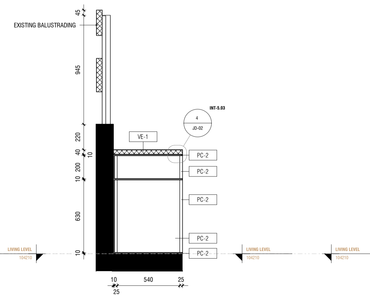
3 INT-5.03 SECTION 1 1:20
